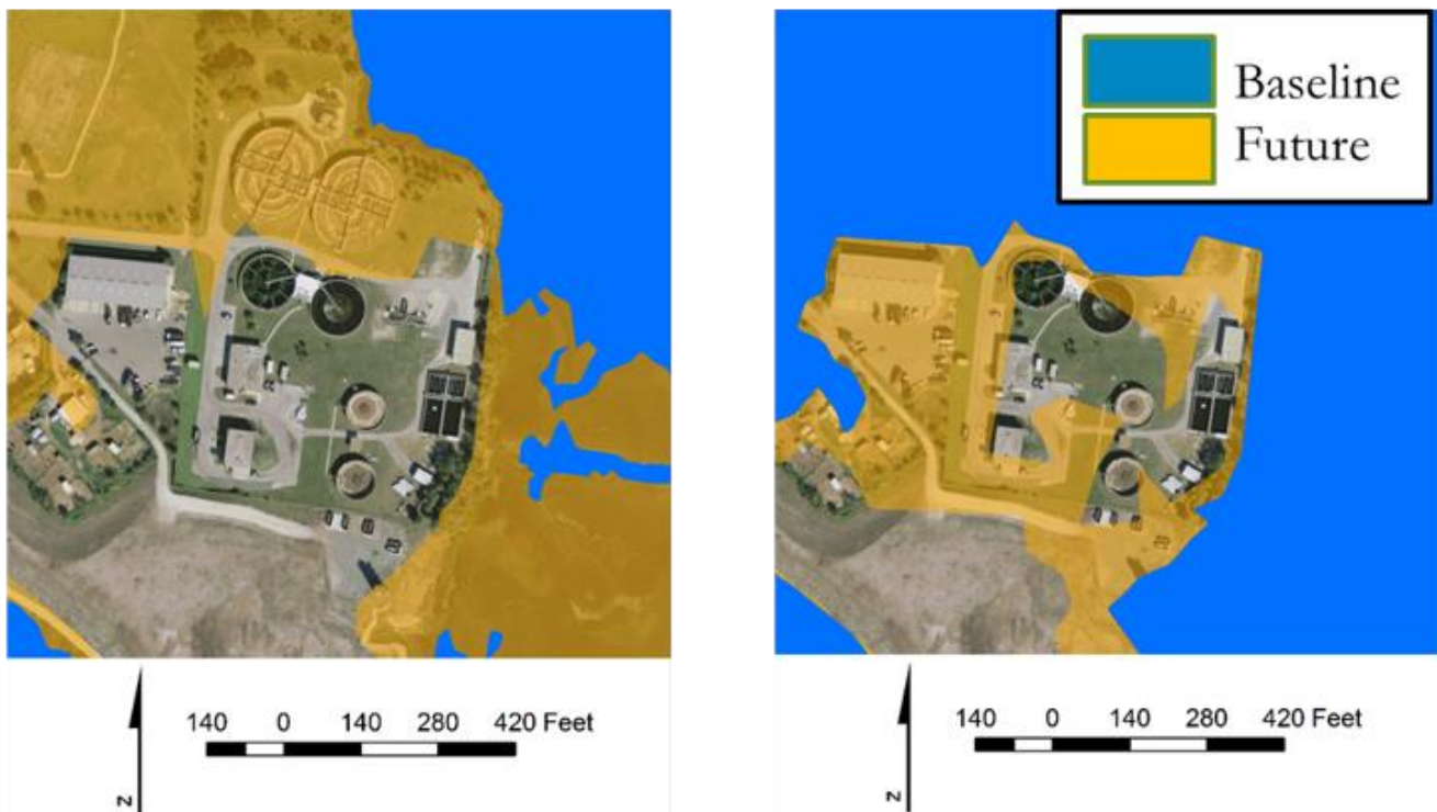
Figure 16. Wasterwater treatment plant structure exposure tipping points to MHHW + 5 ft SLR (left) and to the 1% Event + 1.0 ft SLR (right).
