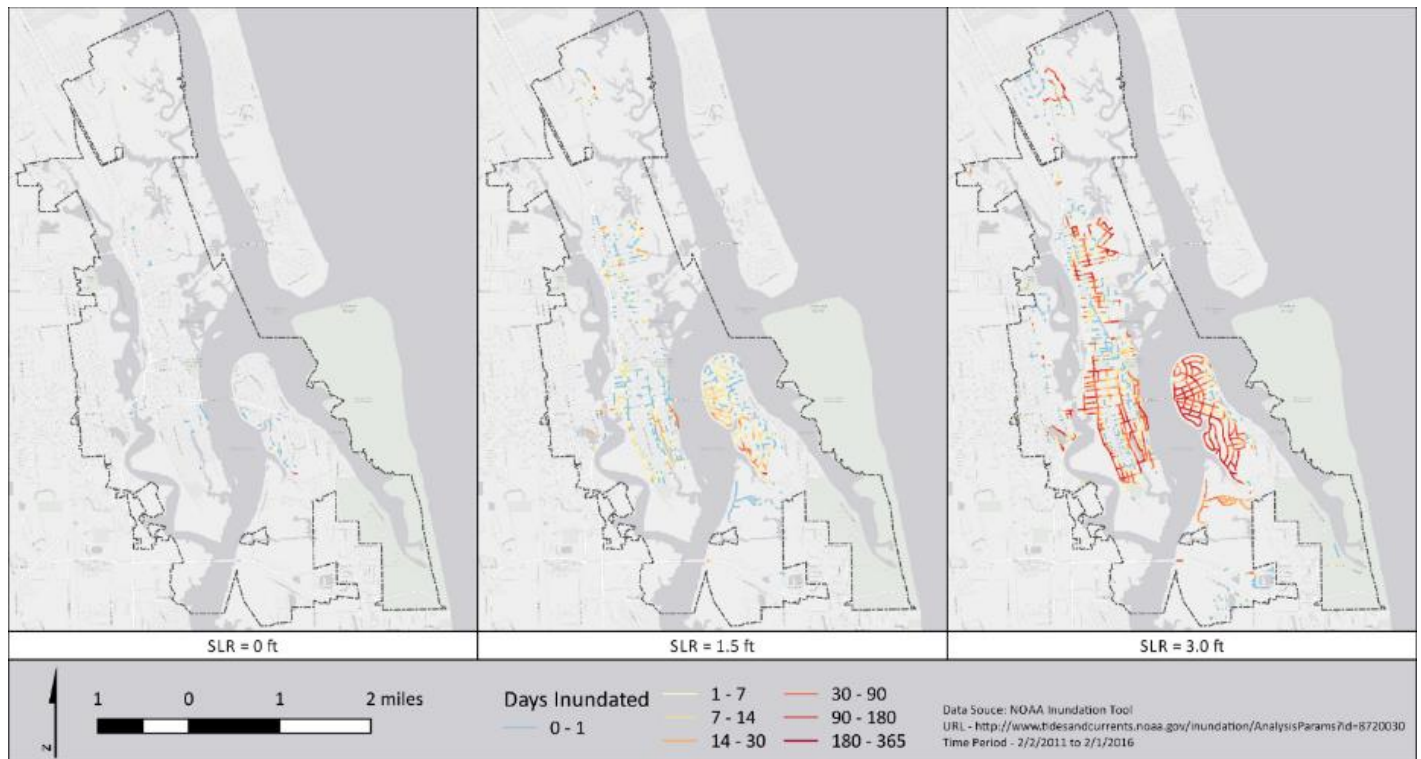
Figure 8. The vulnerability of the road network to nuisance flooding increases significantly from present day conditions with 1.5 and 3 ft of SLR.
