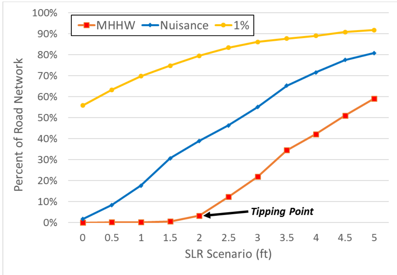
Figure 7. Percent of road network affected by MHHW, nuisance, and the 1% flood level for each SLR increment.
