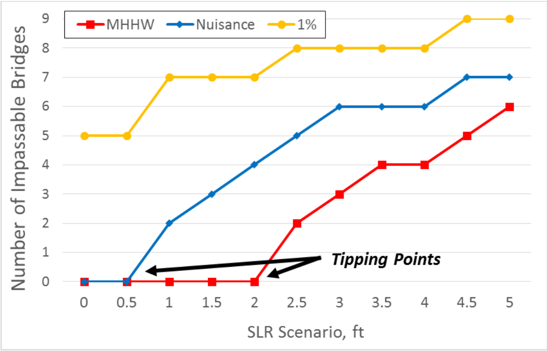
Figure 9. Number of bridges transitioned to impassable by MHHW, nuisance, and the 1% flood level in each SLR scenario.
