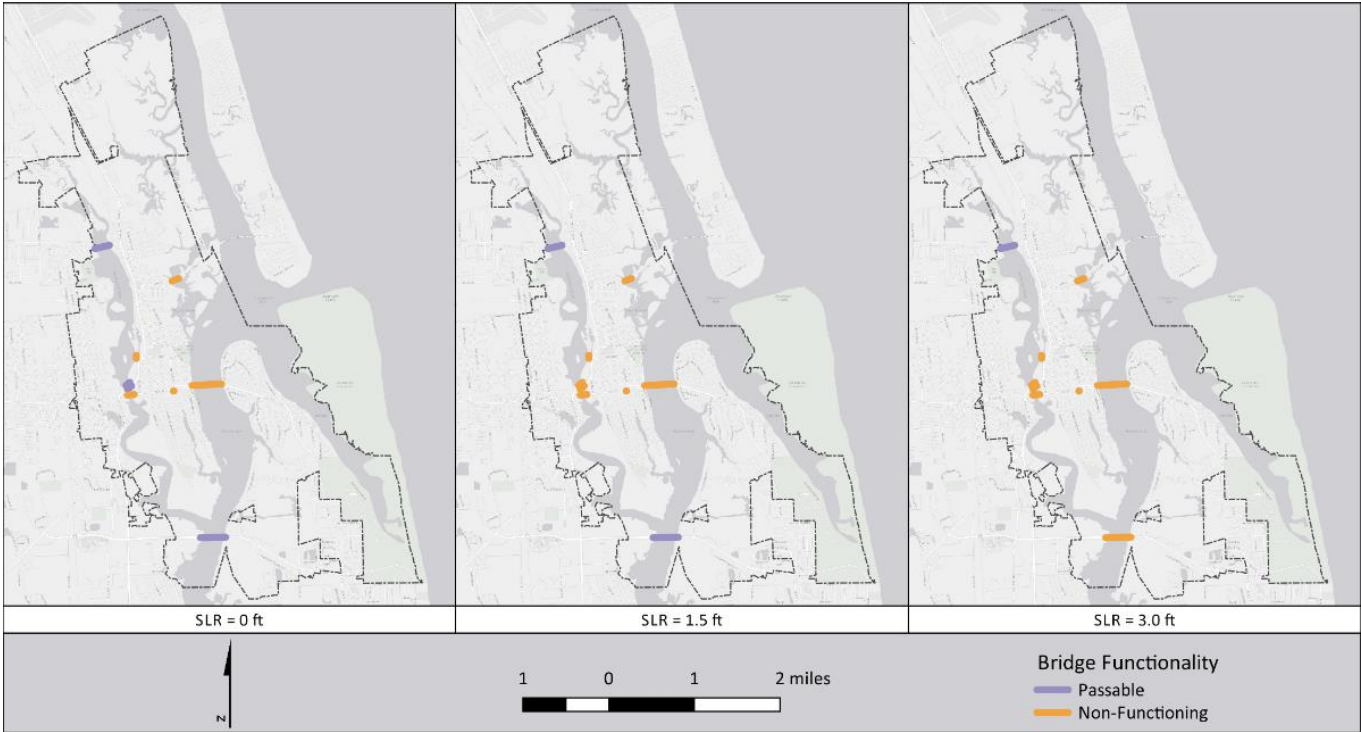
Figure 10. Bridge vulnerability to the nuisance flood event with SLR.
