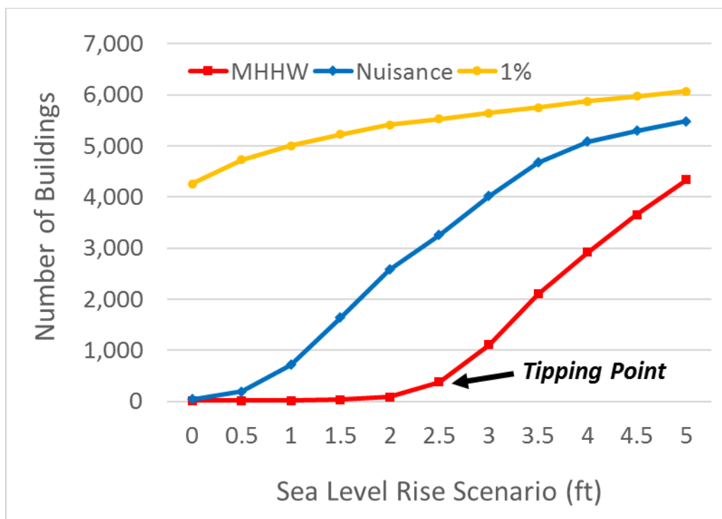
Figure 12. Number of buildings (commercial, residential and municipal) affected by MHHW, nuisance, and the 1% flood level in each SLR scenario.
