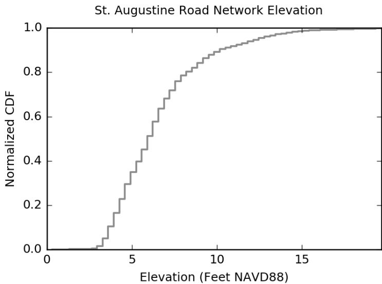
Figure 21. St. Augustine road network elevation, cumulative distribution function.
